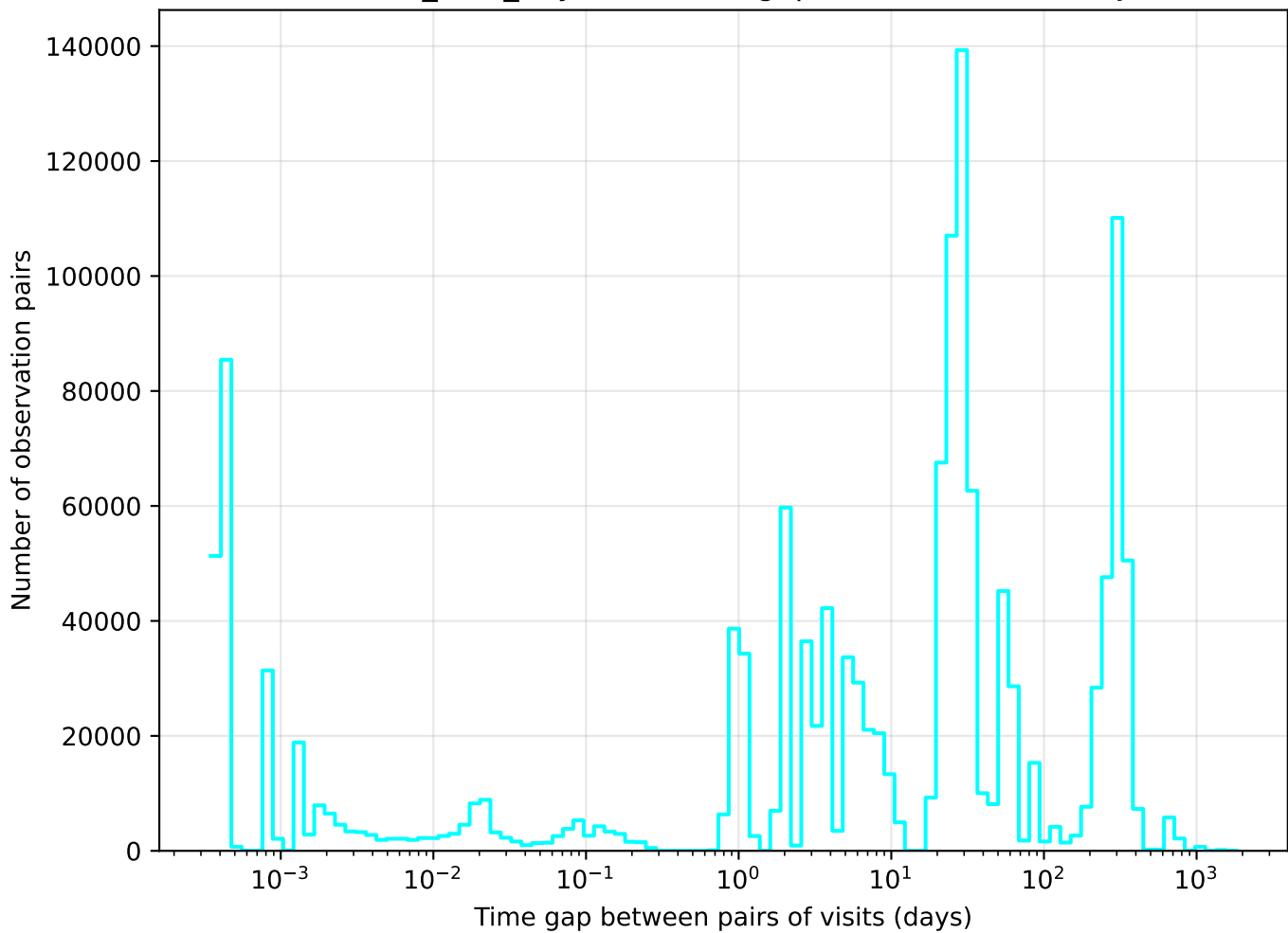
baseline_v2.1_10yrs u band: Tgaps observationStartMJD
