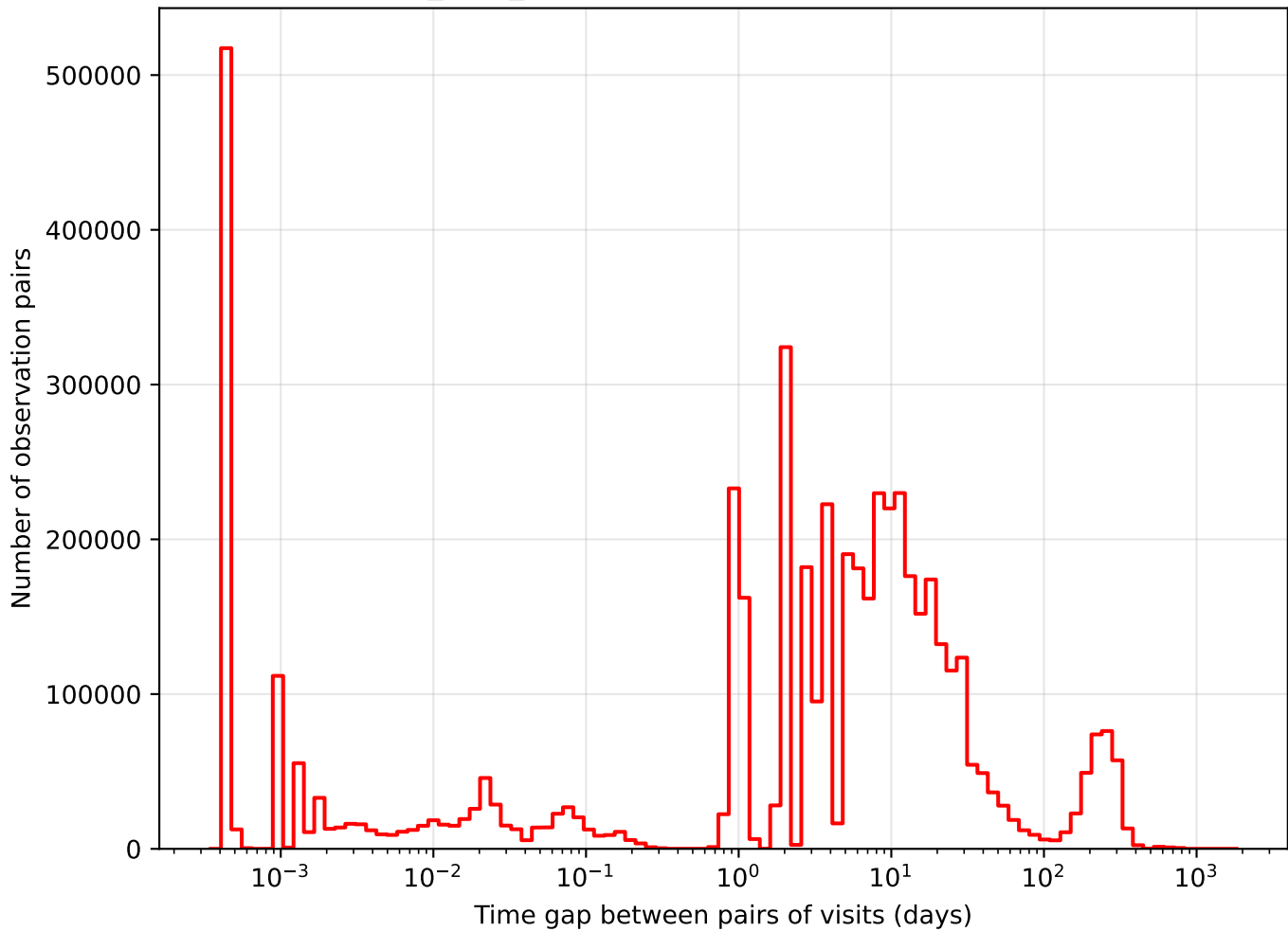
baseline_v2.1_10yrs i band: Tgaps observationStartMJD
