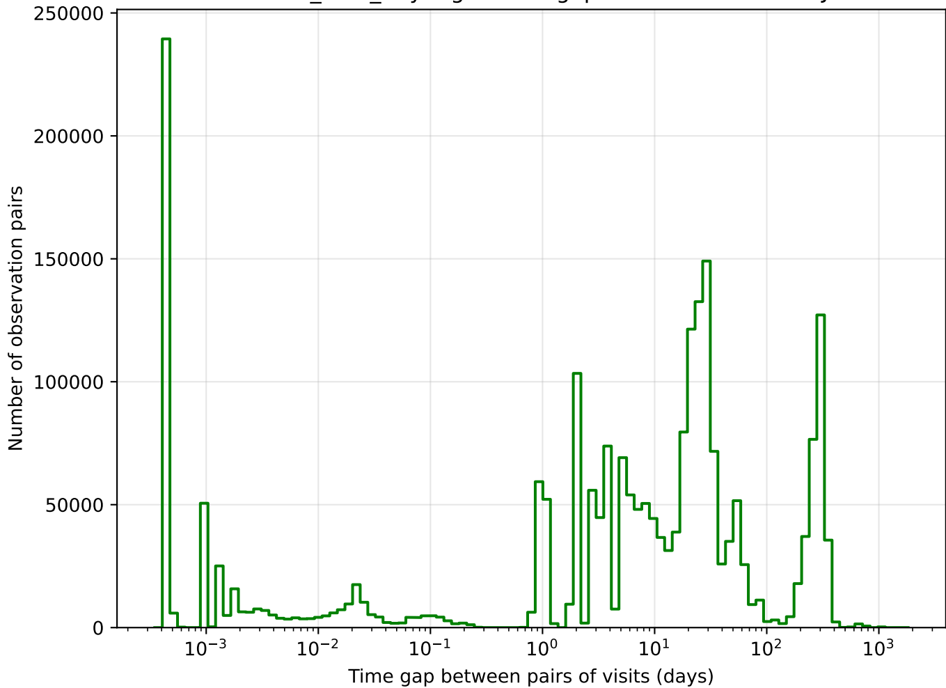
baseline_v2.1_10yrs g band: Tgaps observationStartMJD
