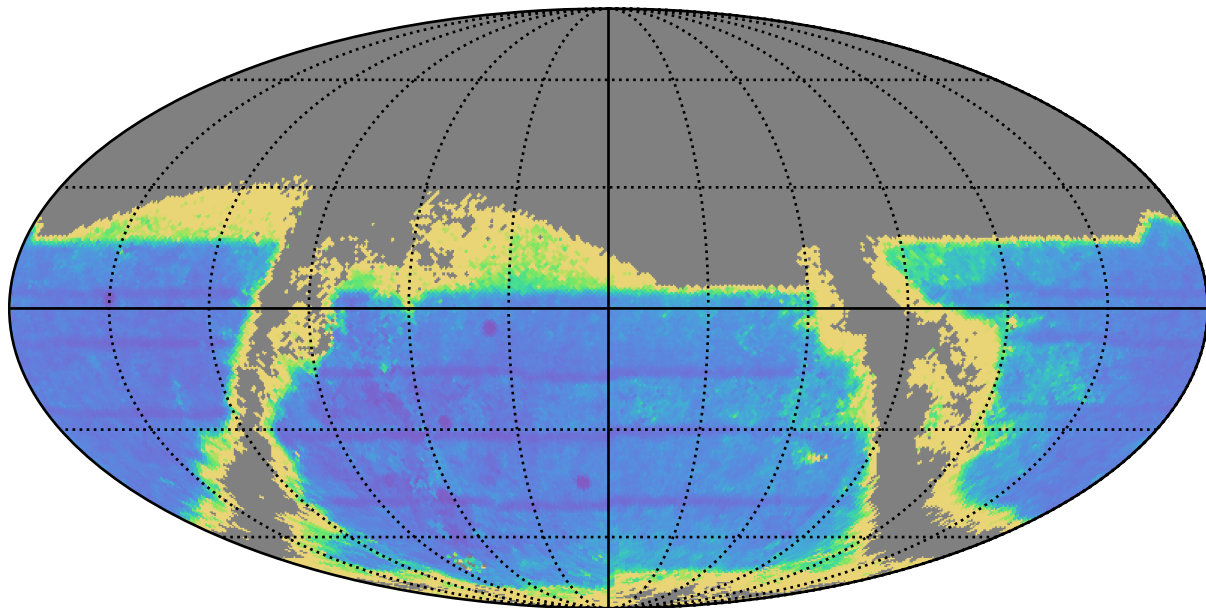
baseline_v2.1_10yrs : TDC_precision
