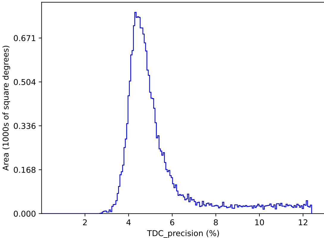
baseline_v2.1_10yrs : TDC_precision
