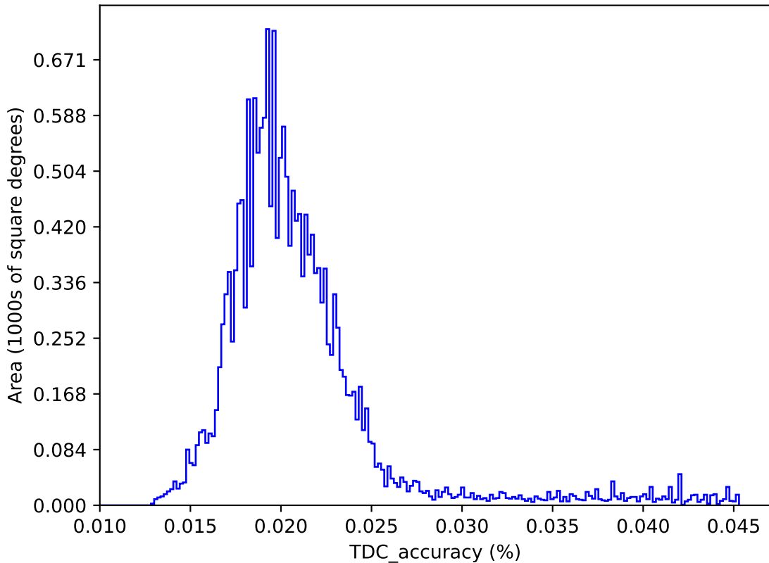
baseline_v2.1_10yrs : TDC_accuracy
