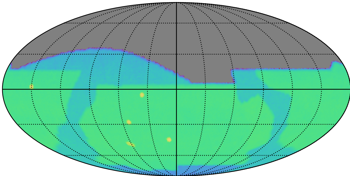
baseline_v2.1_10yrs z: SurfaceBrightLimit
