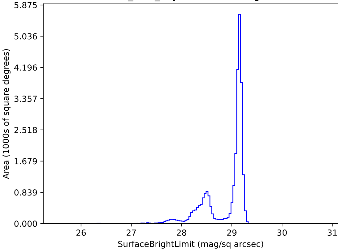
baseline_v2.1_10yrs z: SurfaceBrightLimit
