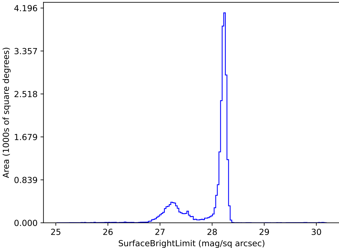
baseline_v2.1_10yrs y: SurfaceBrightLimit
