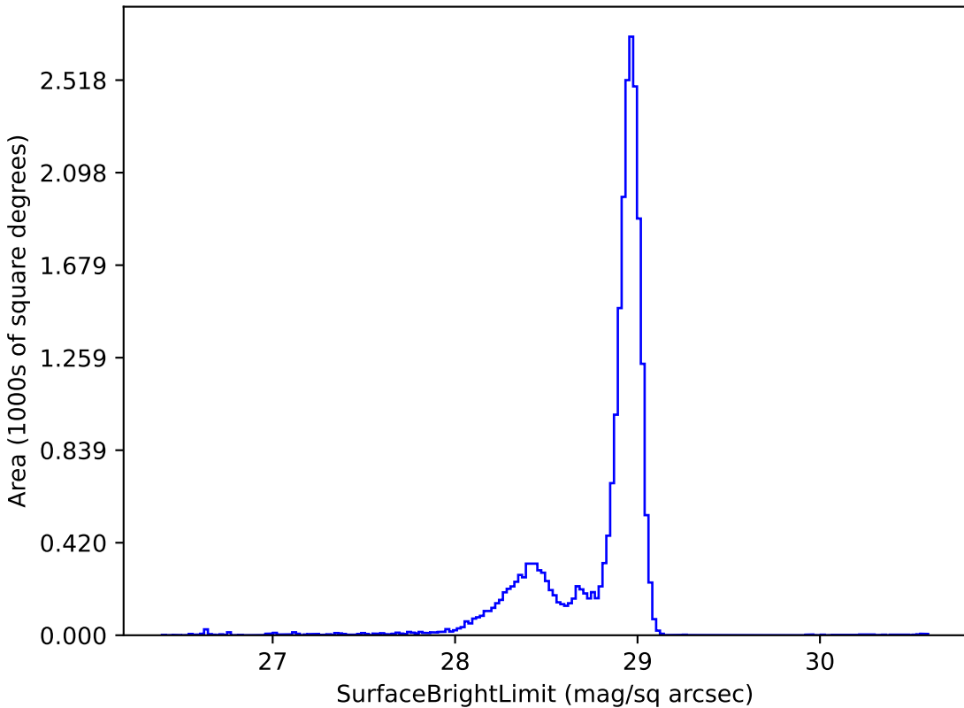
baseline_v2.1_10yrs u: SurfaceBrightLimit
