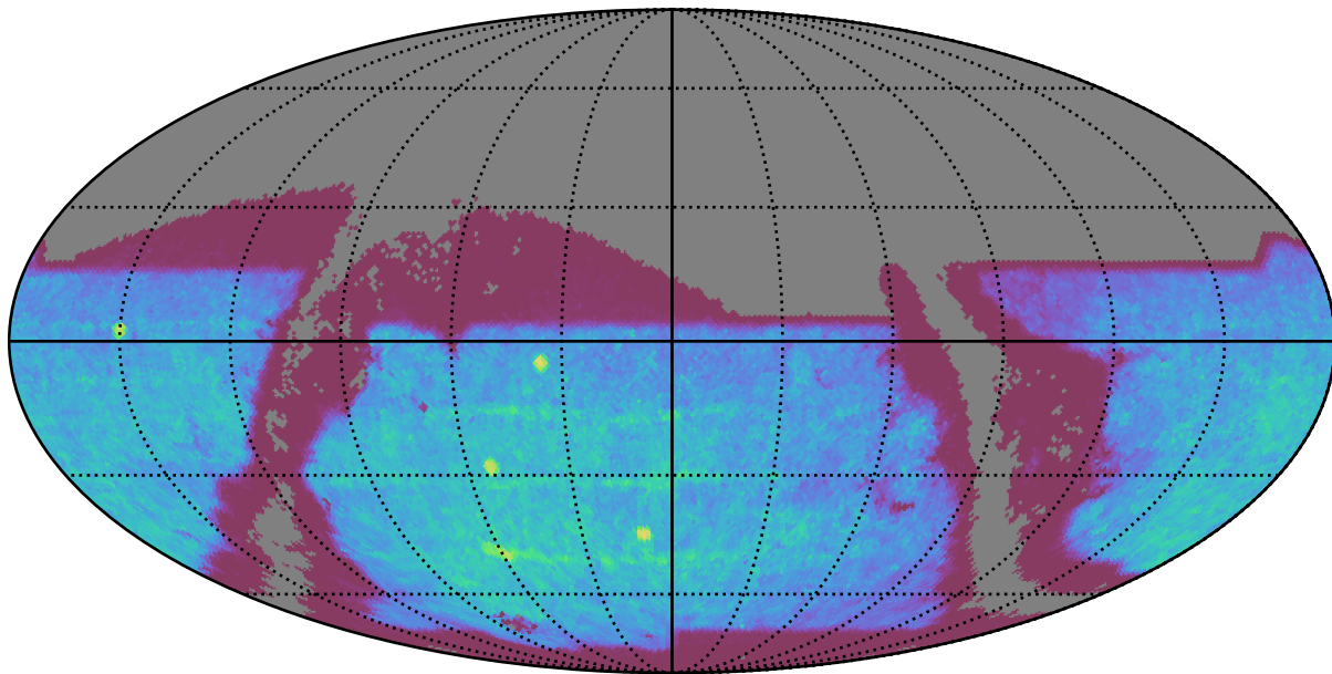
baseline_v2.1_10yrs : SNSLMetric
