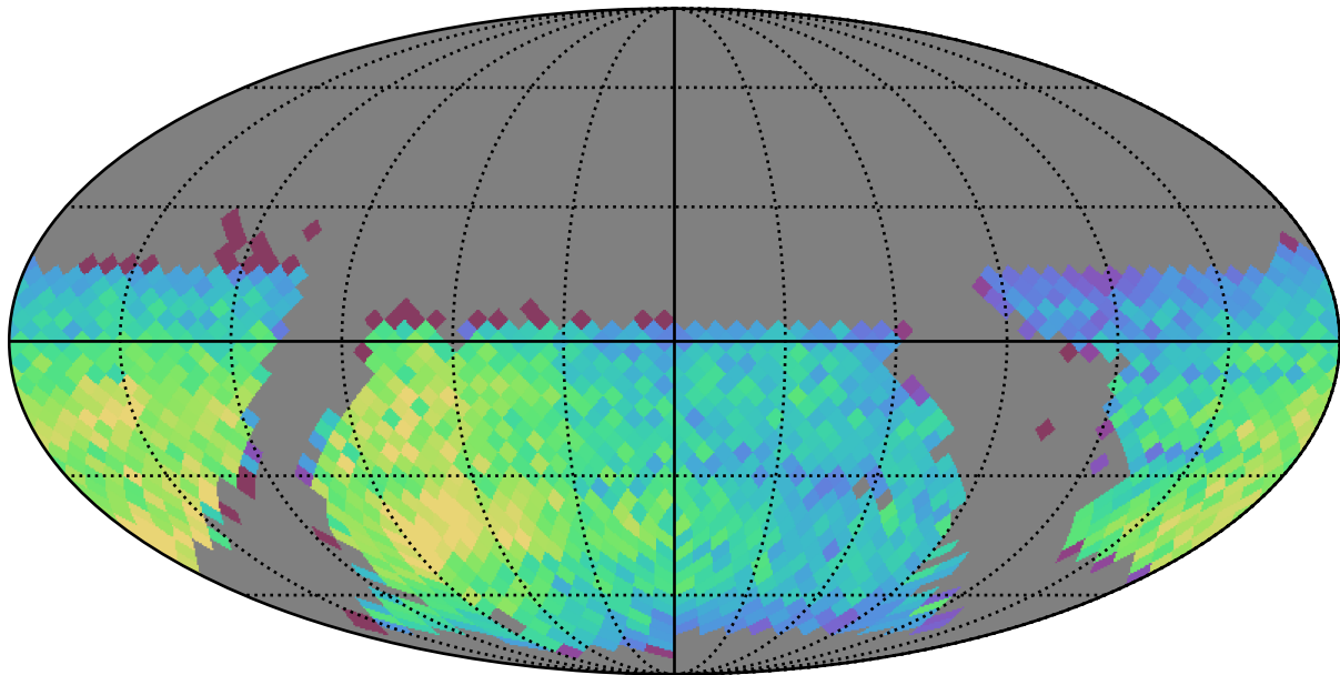
baseline_v2.1_10yrs DDF excluded: SNNSNMetric_reducen_sn
