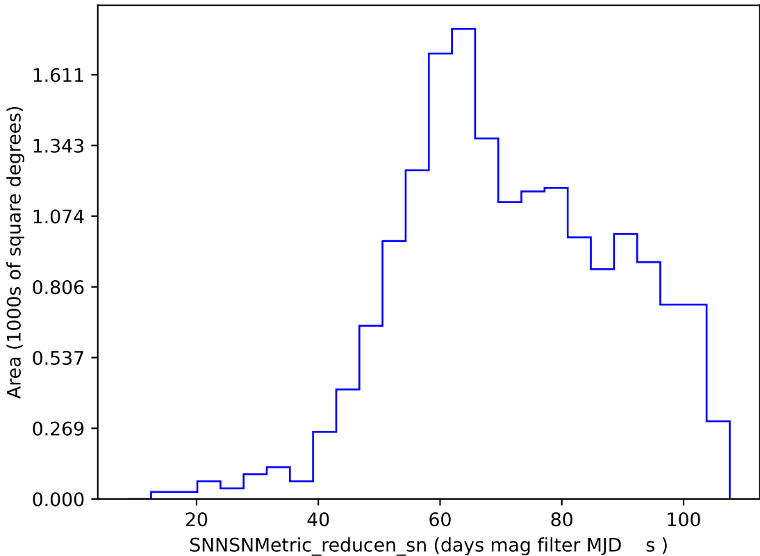
baseline_v2.1_10yrs DDF excluded: SNNSNMetric_reducen_sn
