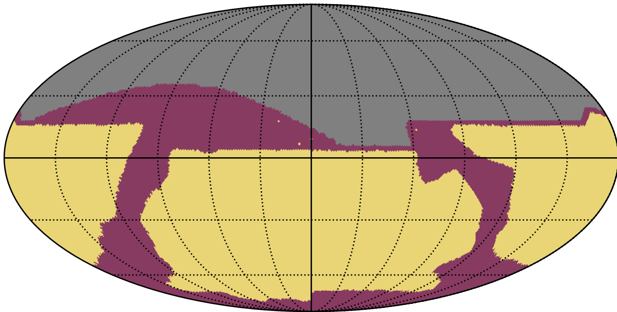
baseline_v2.1_10yrs : RapidRevisits
