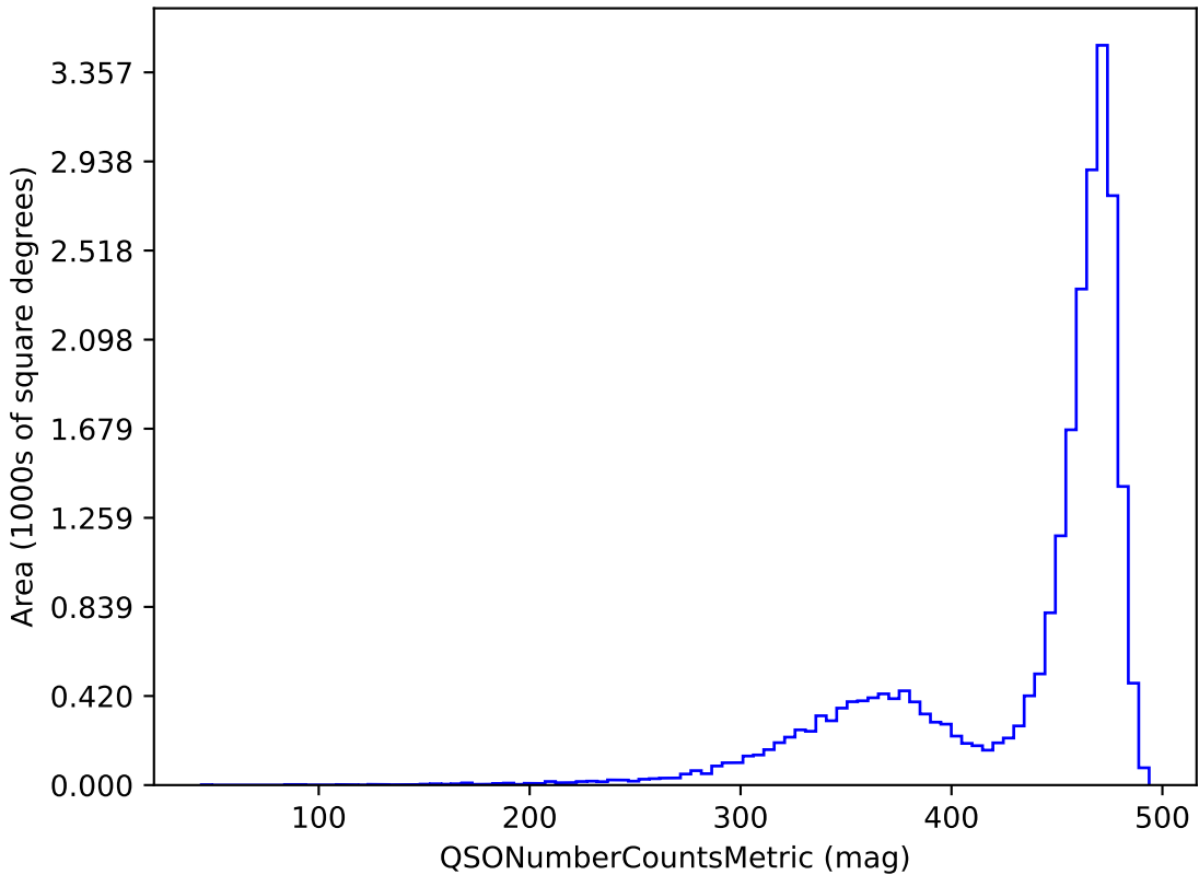
baseline_v2.1_10yrs z band and non-DD: QSONumberCountsMetric
