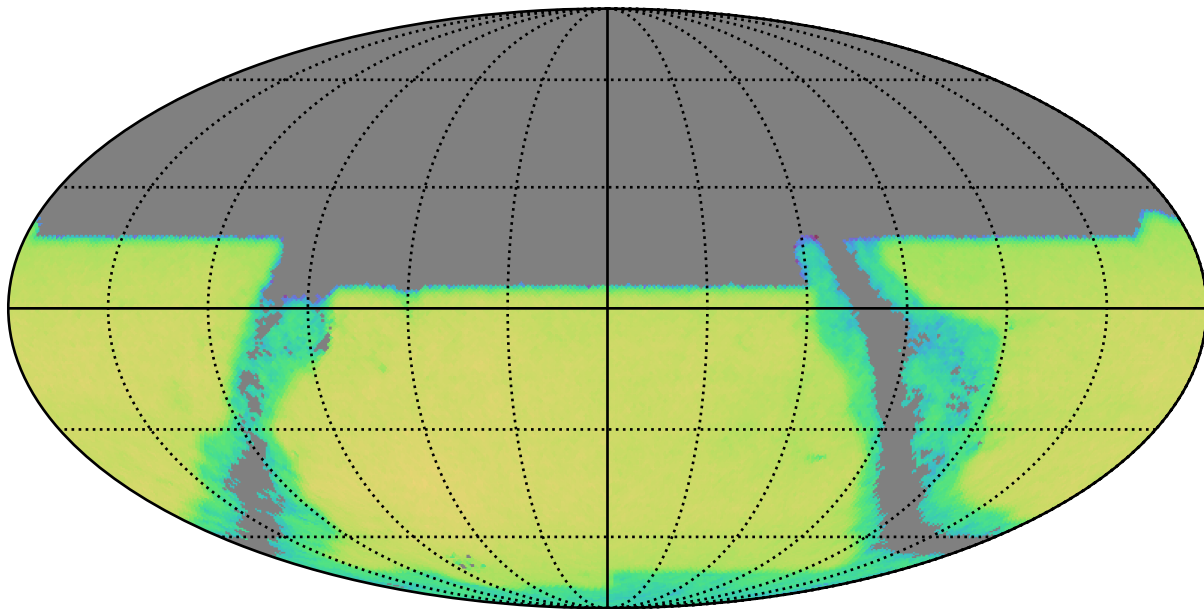
baseline_v2.1_10yrs y band and non-DD: QSONumberCountsMetric
