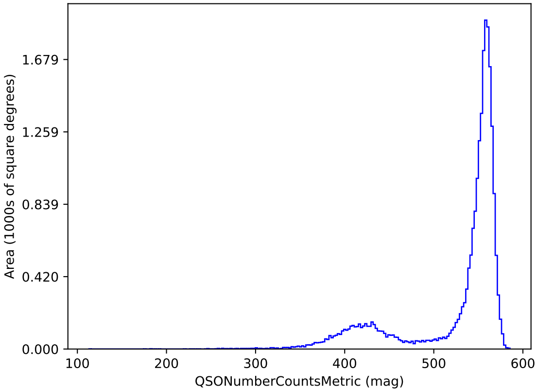
baseline_v2.1_10yrs y band and non-DD: QSONumberCountsMetric
