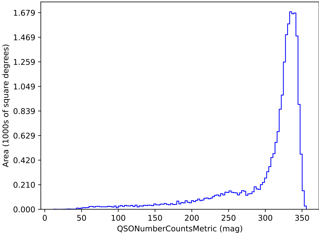
baseline_v2.1_10yrs u band and non-DD: QSONumberCountsMetric
