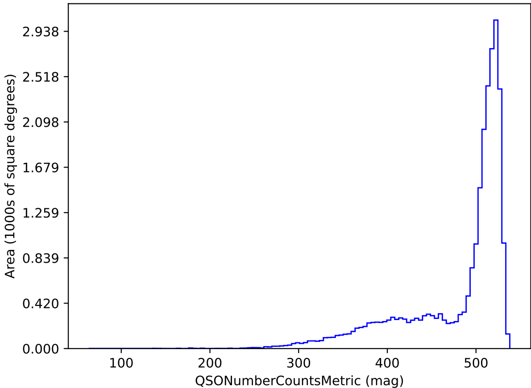
baseline_v2.1_10yrs r band and non-DD: QSONumberCountsMetric
