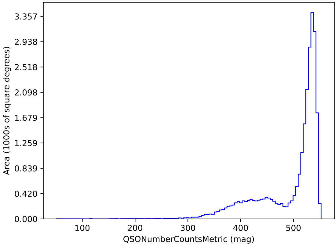
baseline_v2.1_10yrs i band and non-DD: QSONumberCountsMetric
