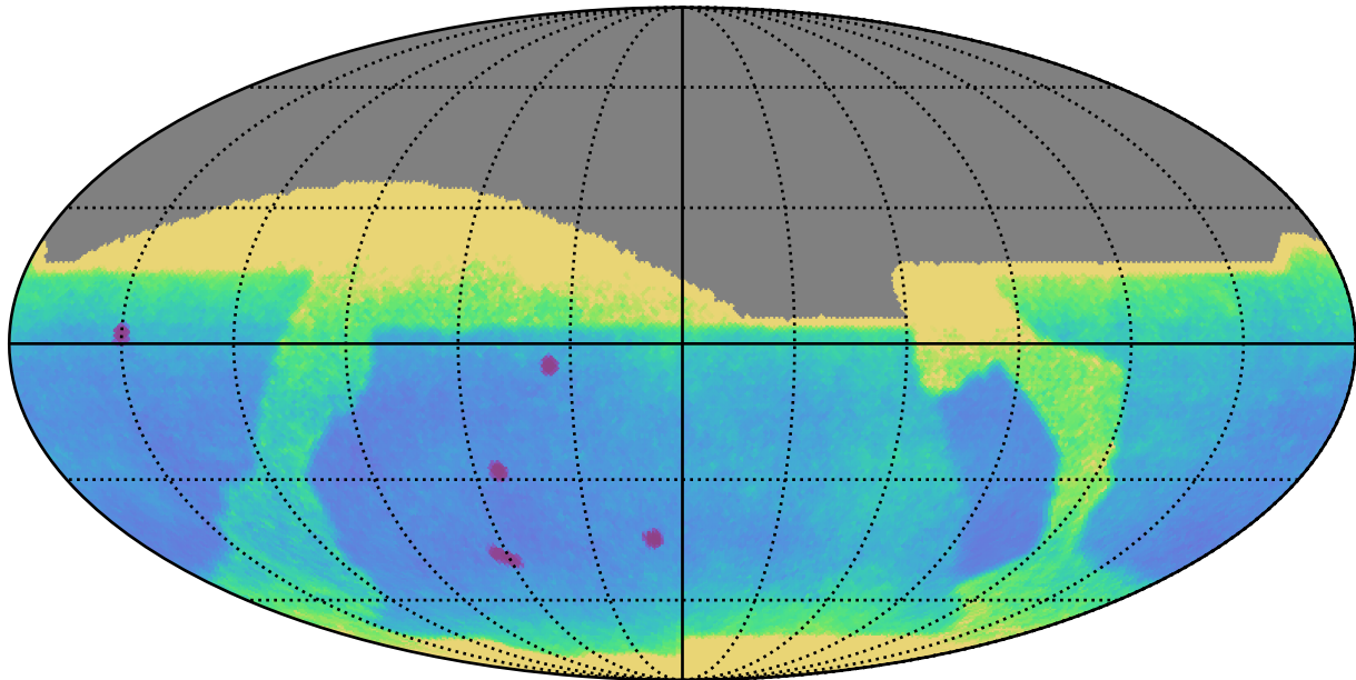
baseline_v2.1_10yrs : Proper Motion Uncert @ 24.0
