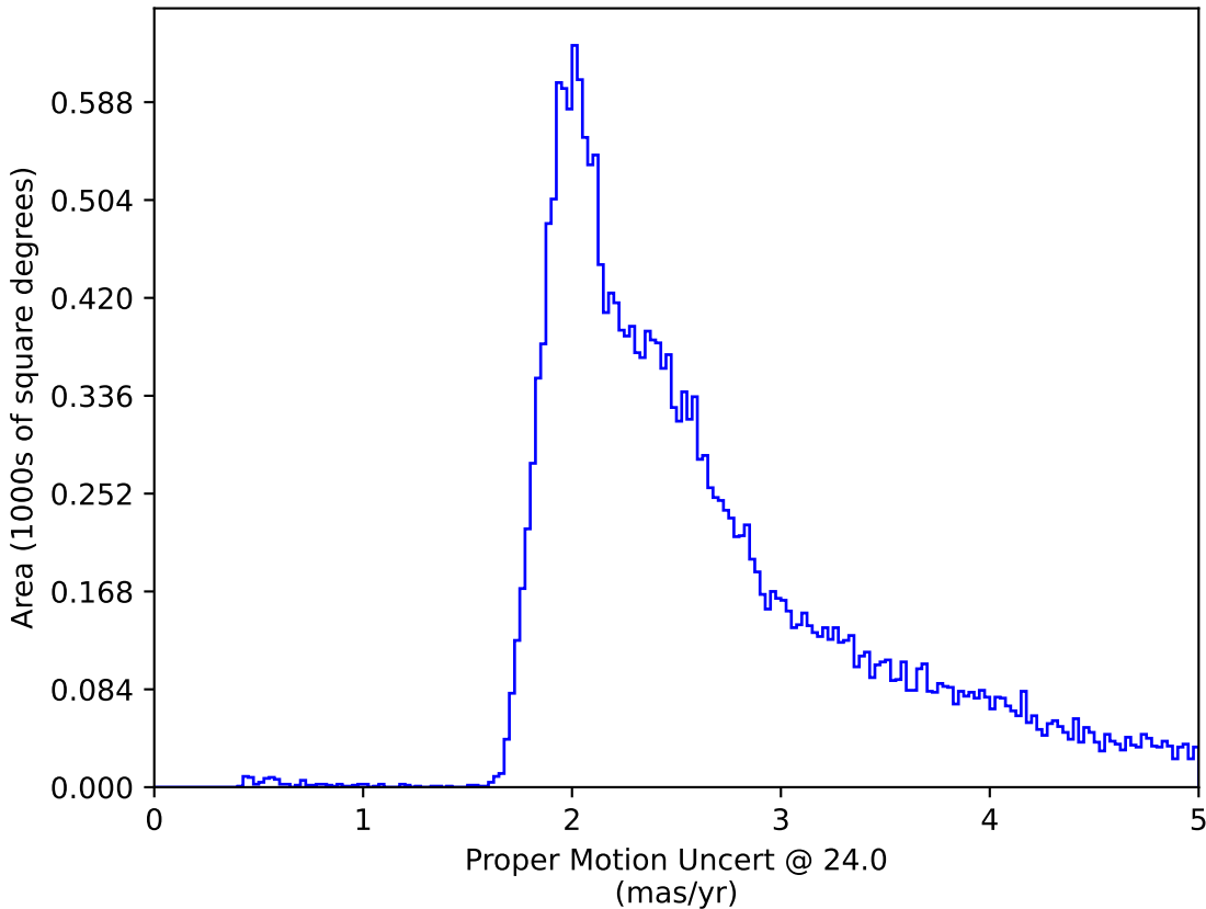
baseline_v2.1_10yrs : Proper Motion Uncert @ 24.0
