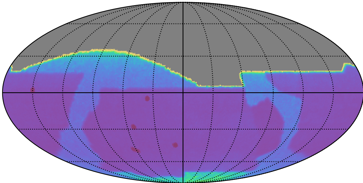
baseline_v2.1_10yrs : Proper Motion Uncert @ 20.5
