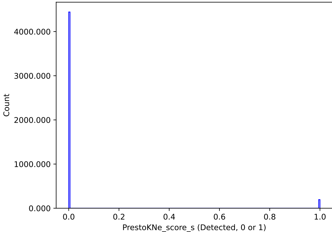
baseline_v2.1_10yrs : PrestoKNe_score_s
