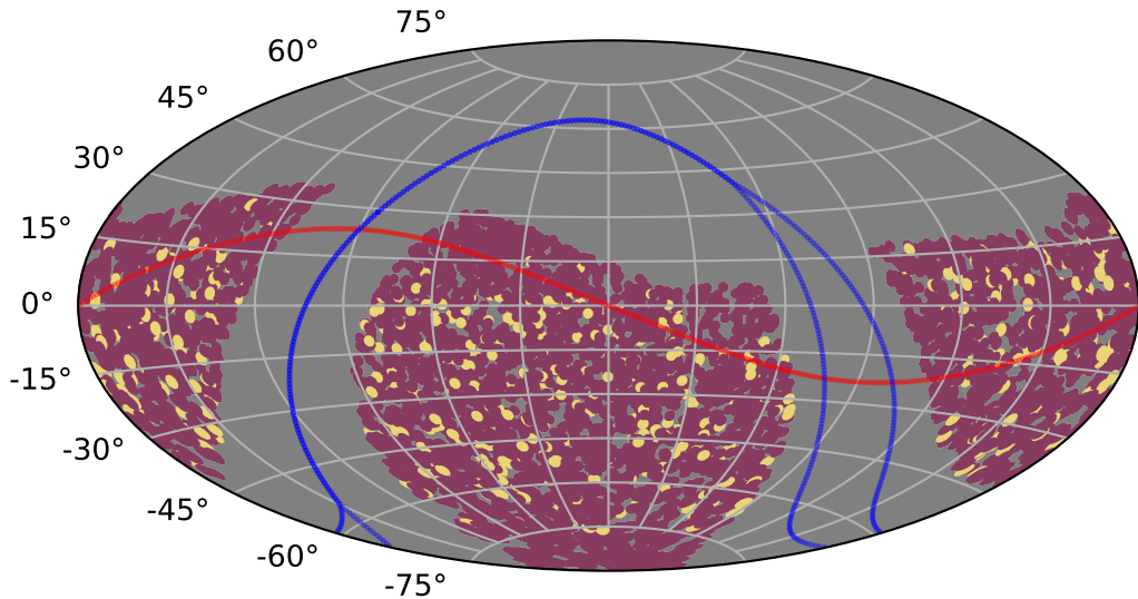
baseline_v2.1_10yrs : PrestoKNe_presto_color_detect
