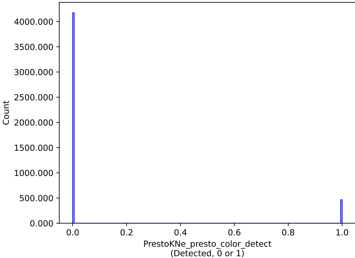
baseline_v2.1_10yrs : PrestoKNe_presto_color_detect
