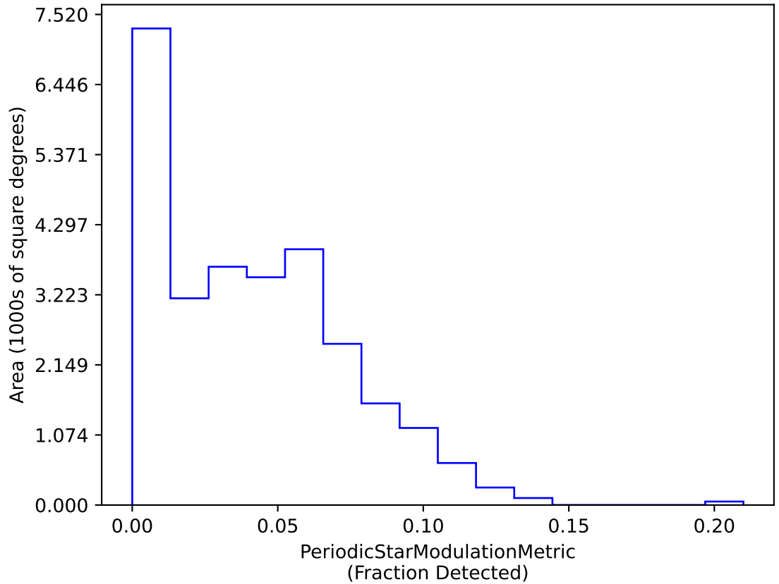
baseline_v2.1_10yrs dm 20 interval 15 R Rc Year 1-2: PeriodicStarModulationMetric
