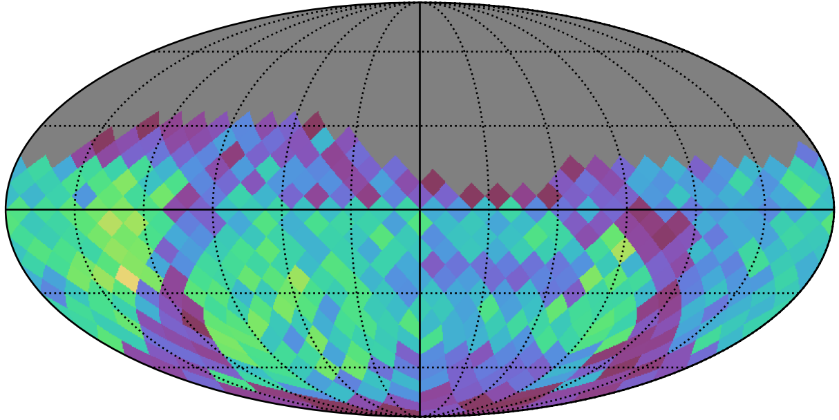
baseline_v2.1_10yrs dm 18 interval 30 RRc Year 1-2: PeriodicStarModulationMetric
