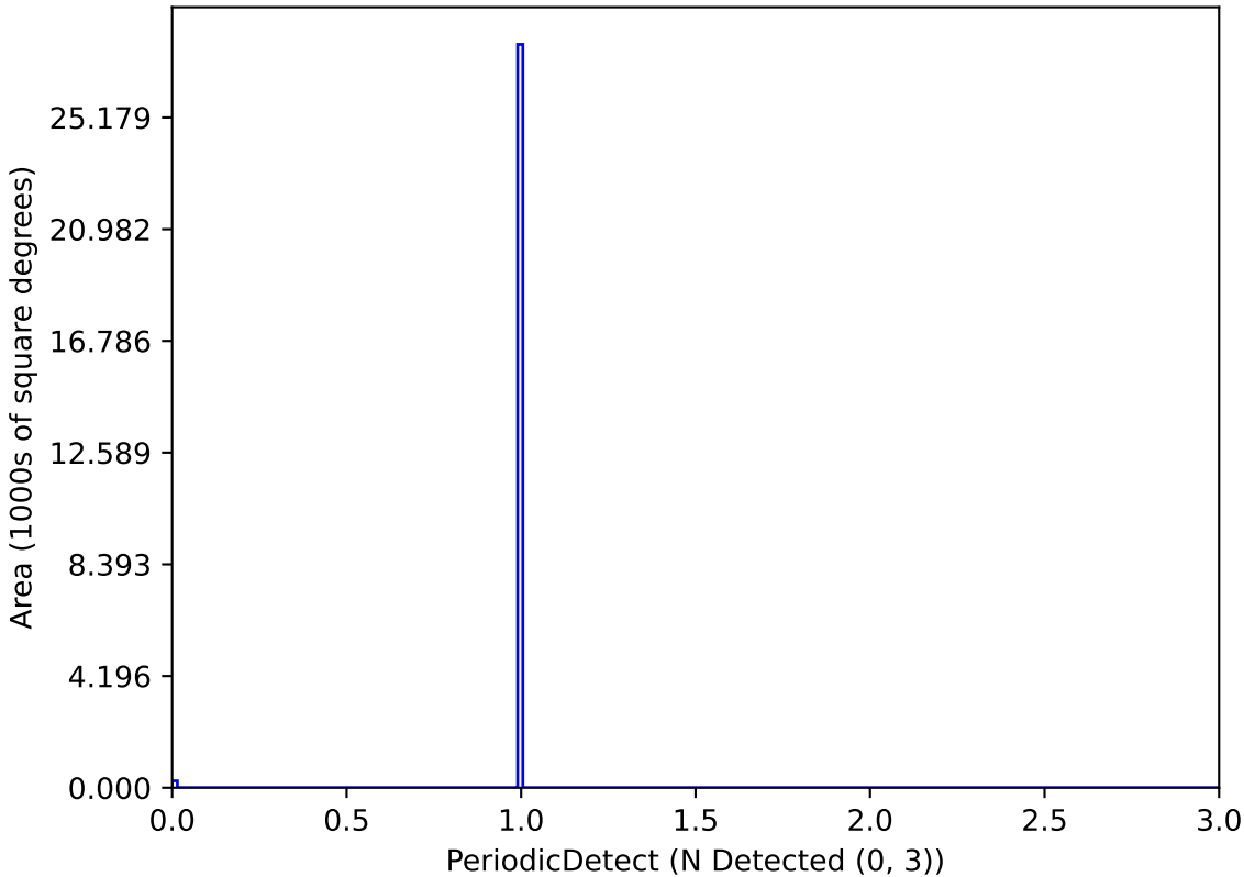
baseline_v2.1_10yrs P_2.0_Mag_24_Amp_0.05-0.1-1: PeriodicDetect
