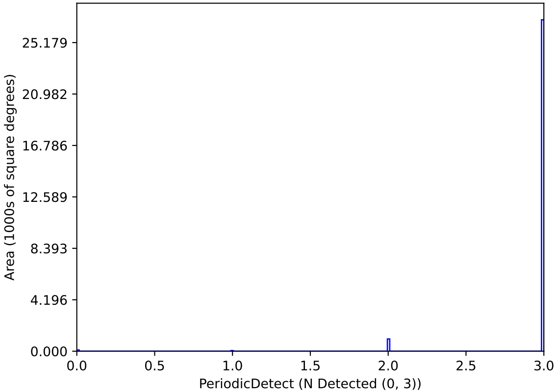
baseline_v2.1_10yrs P_2.0_Mag_21_Amp_0.05-0.1-1: PeriodicDetect
