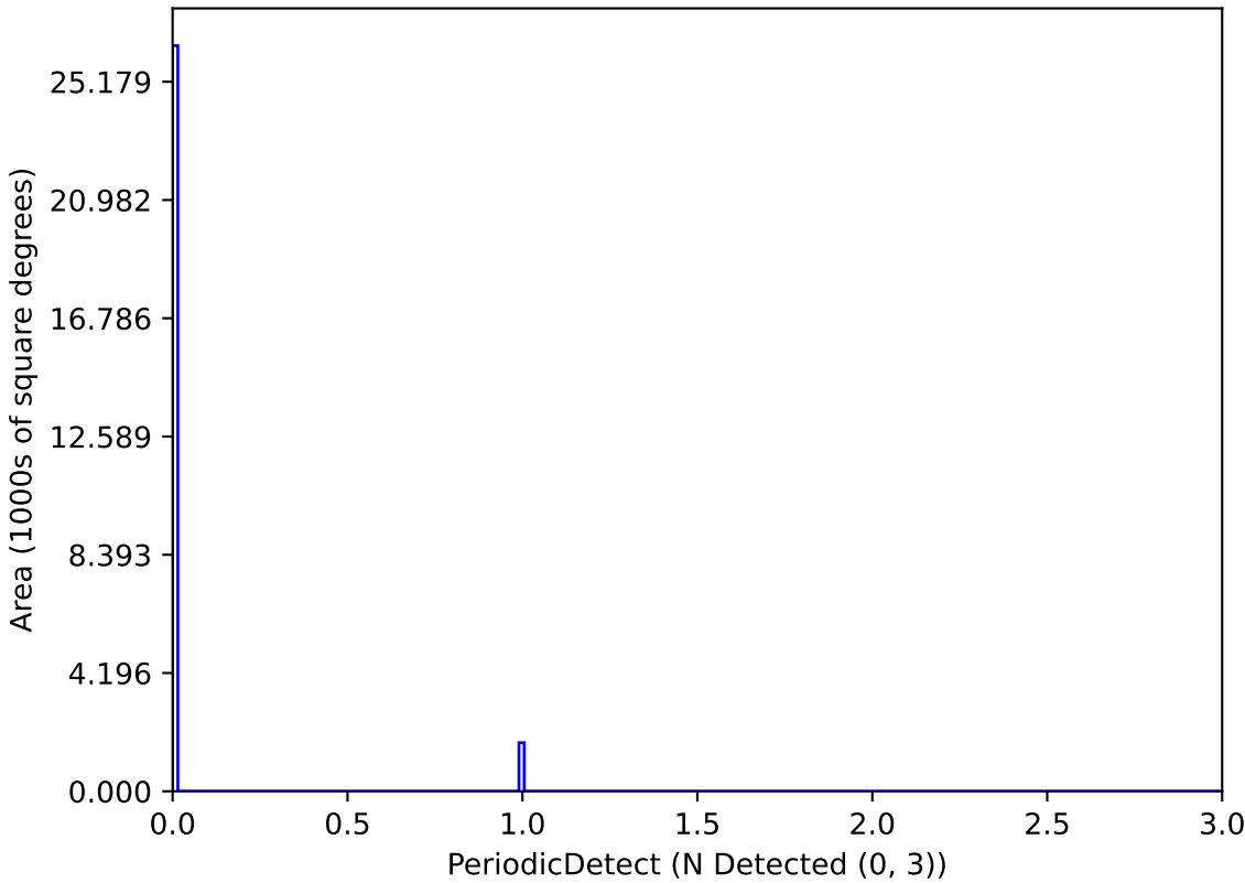
baseline_v2.1_10yrs P_1.0_Mag_24_Amp_0.05-0.1-1: PeriodicDetect
