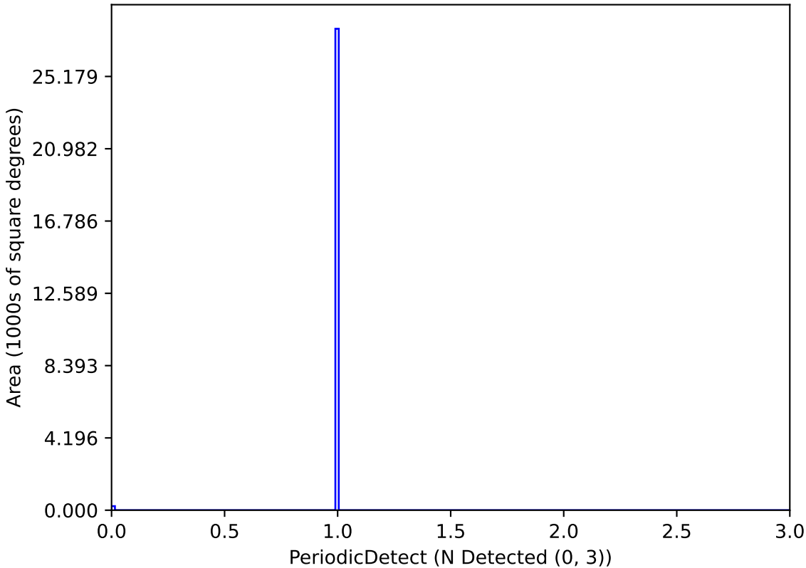
baseline_v2.1_10yrs P_0.5_Mag_24_Amp_0.05-0.1-1: PeriodicDetect
