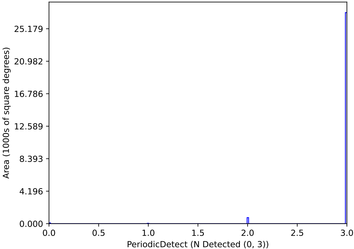
baseline_v2.1_10yrs P_0.5_Mag_21_Amp_0.05-0.1-1: PeriodicDetect
