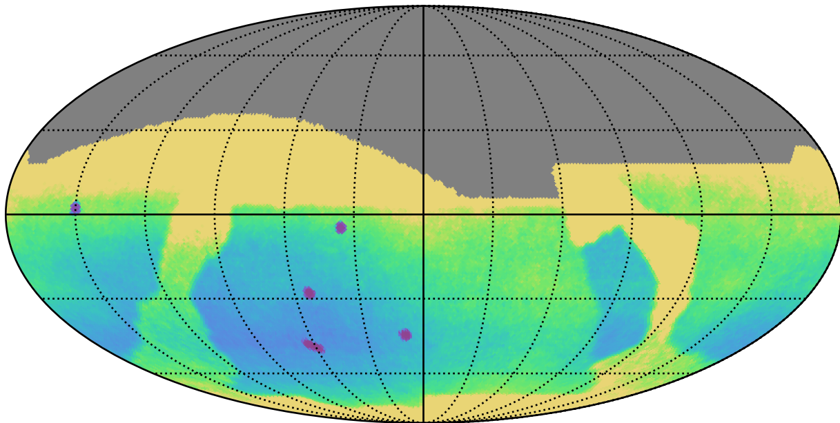
baseline_v2.1_10yrs : Parallax Uncert @ 24.0
