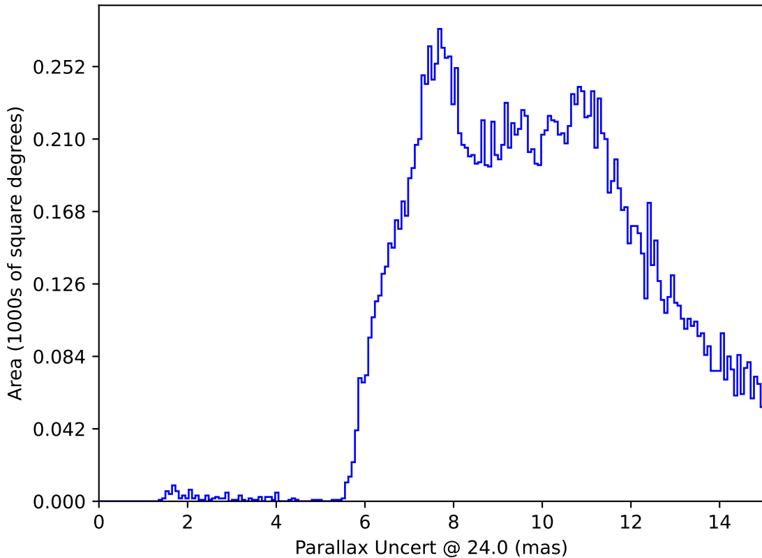
baseline_v2.1_10yrs : Parallax Uncert @ 24.0
