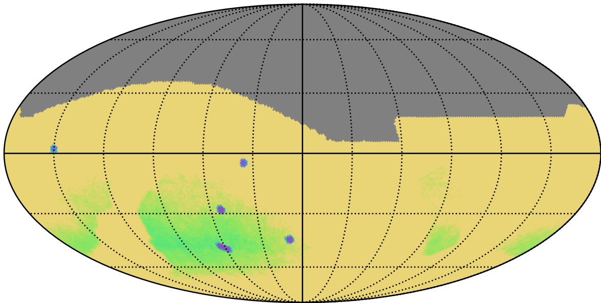
baseline_v2.1_10yrs : Parallax Uncert @ 22.4
