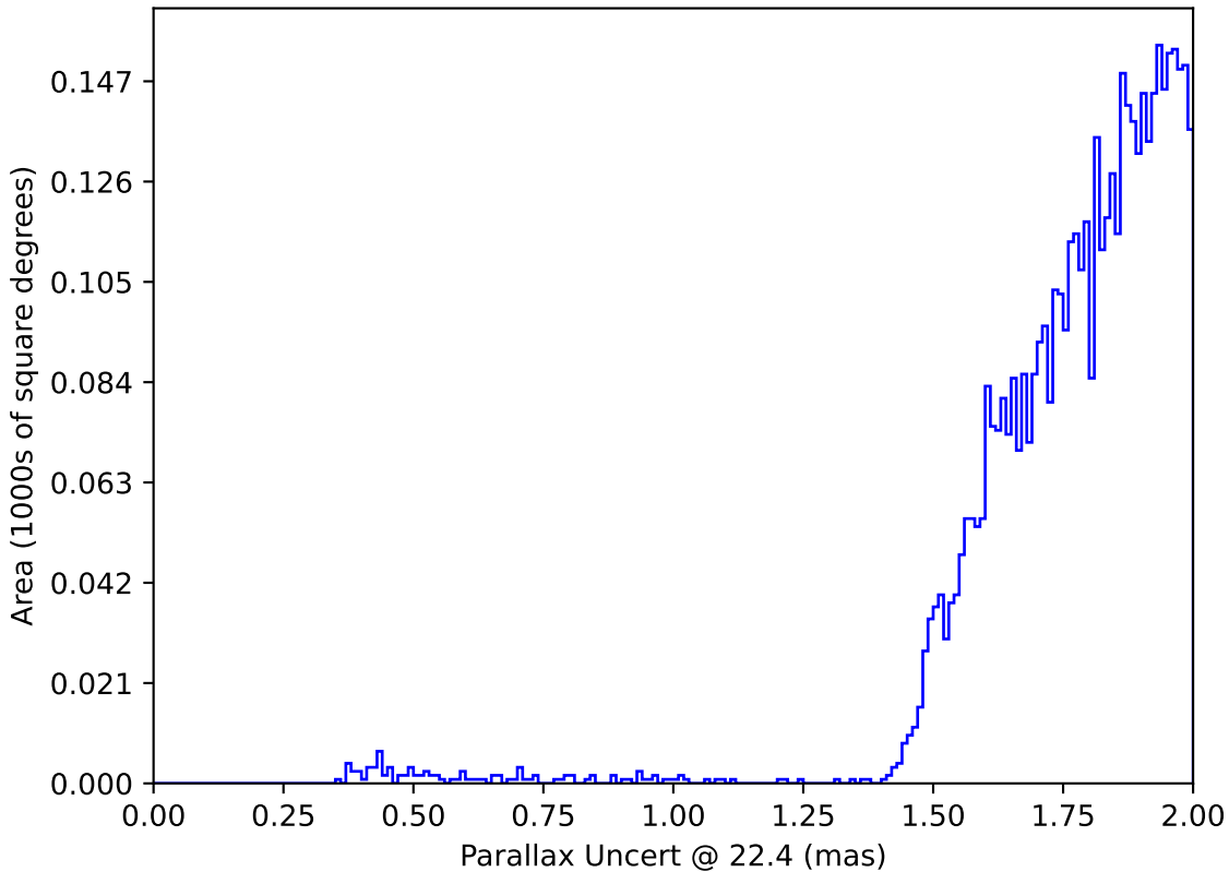
baseline_v2.1_10yrs : Parallax Uncert @ 22.4
