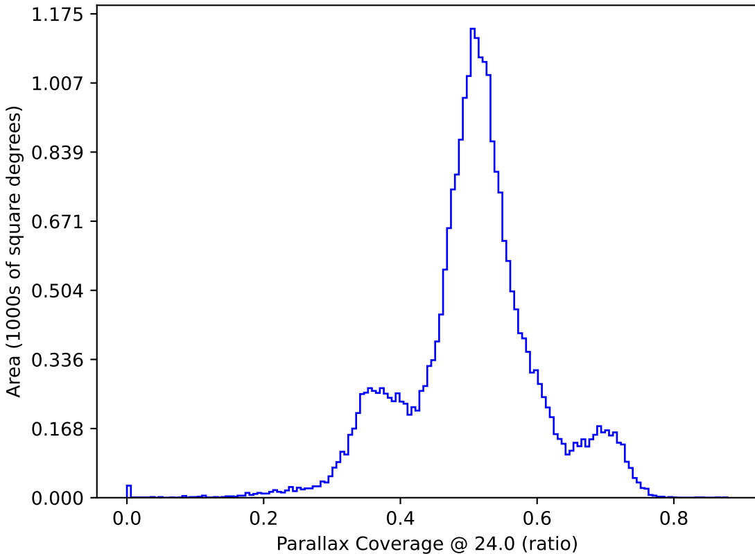
baseline_v2.1_10yrs : Parallax Coverage @ 24.0
