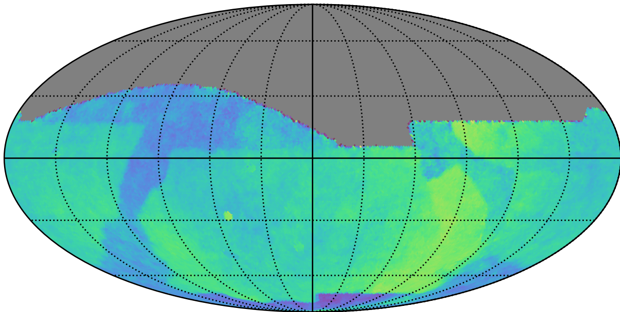
baseline_v2.1_10yrs : Parallax Coverage @ 22.4
