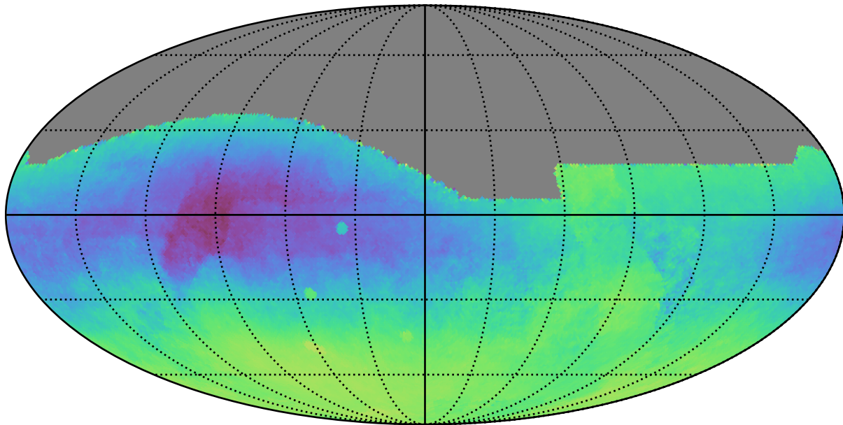
baseline_v2.1_10yrs : Parallax-DCR degeneracy @ 24.0
