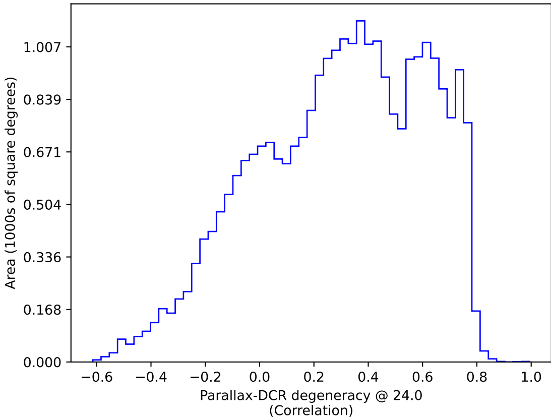
baseline_v2.1_10yrs : Parallax-DCR degeneracy @ 24.0
