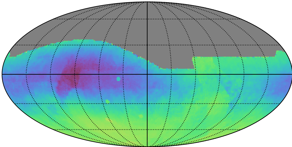
baseline_v2.1_10yrs : Parallax-DCR degeneracy @ 22.4
