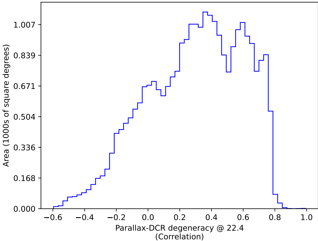
baseline_v2.1_10yrs : Parallax-DCR degeneracy @ 22.4
