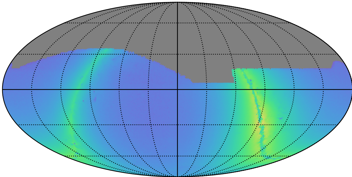
baseline_v2.1_10yrs z: Nstars_no_crowding
