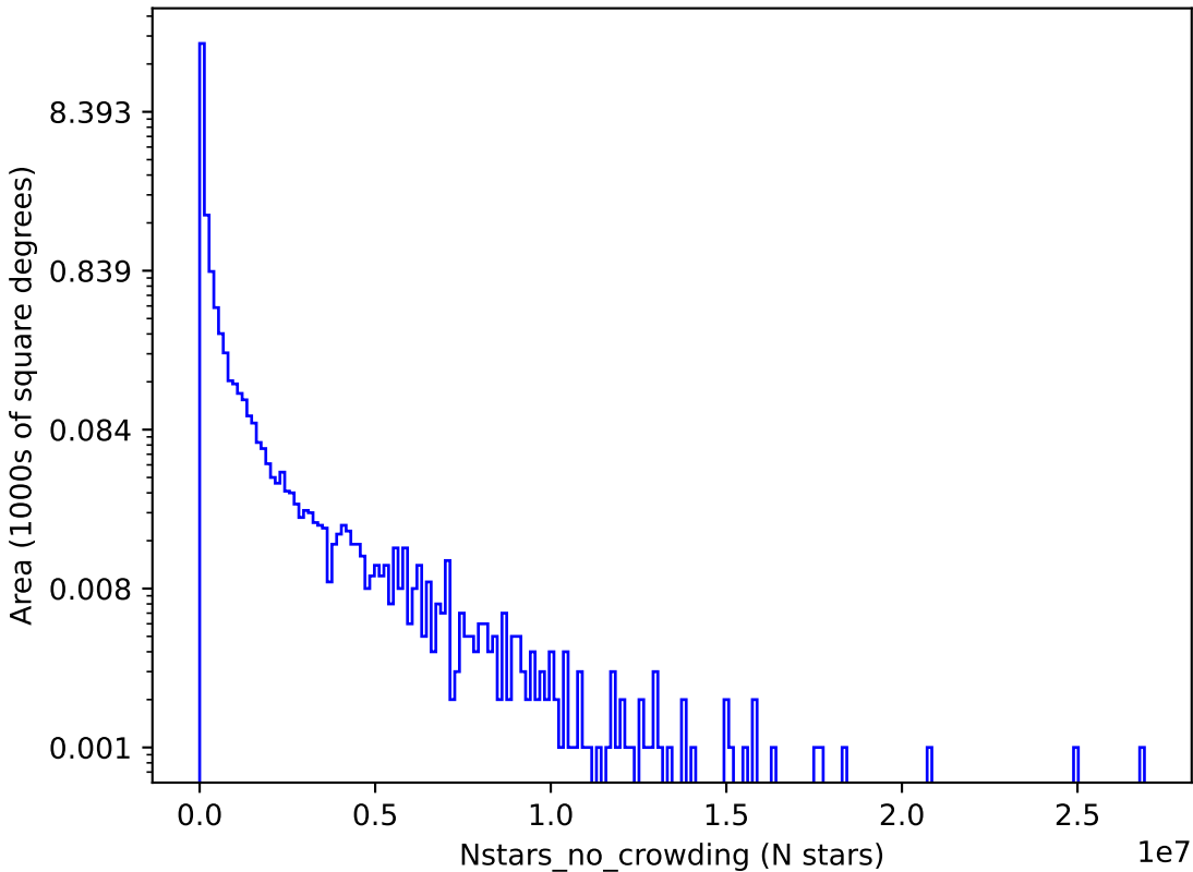
baseline_v2.1_10yrs z: Nstars_no_crowding
