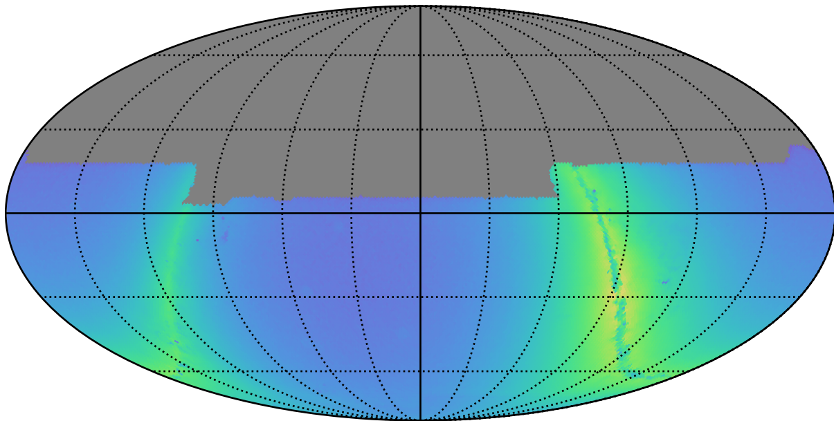
baseline_v2.1_10yrs y: Nstars_no_crowding
