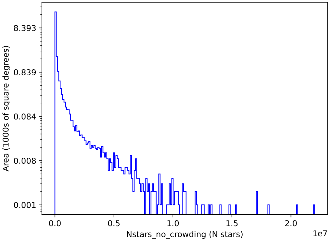
baseline_v2.1_10yrs y: Nstars_no_crowding
