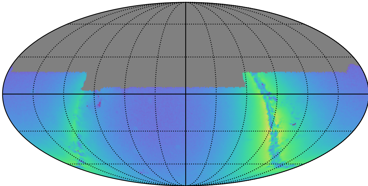
baseline_v2.1_10yrs u: Nstars_no_crowding
