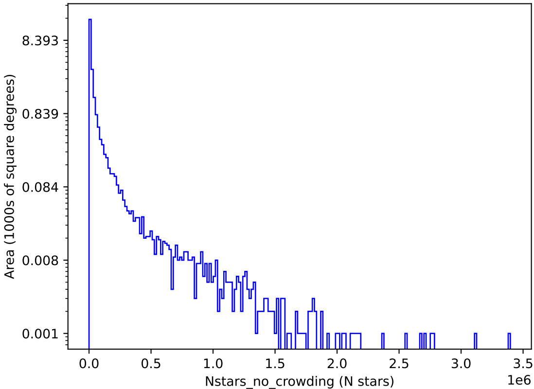
baseline_v2.1_10yrs u: Nstars_no_crowding
