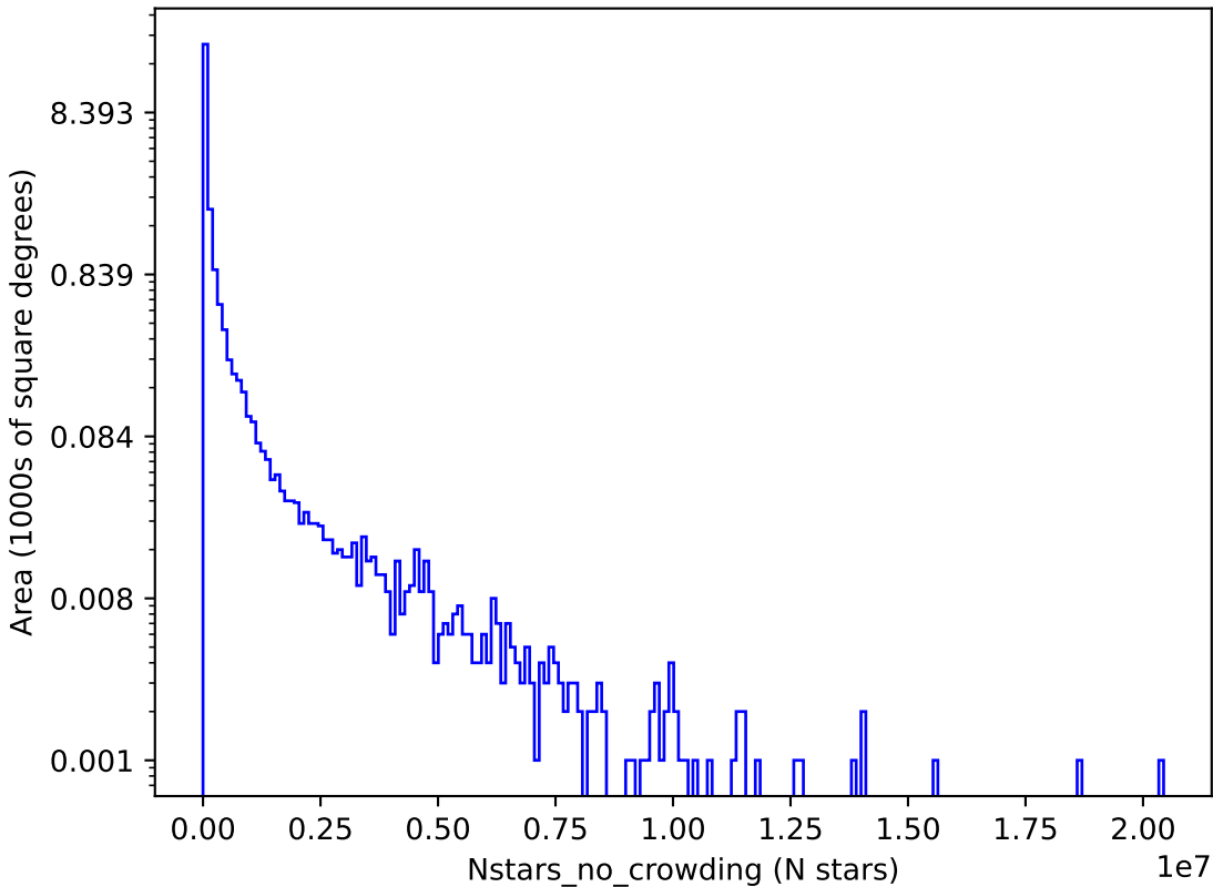
baseline_v2.1_10yrs r: Nstars_no_crowding
